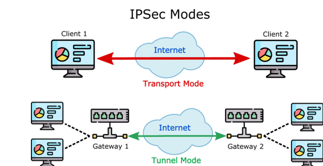
Figure 2: IPsec contains a gateway and a tunnel in order to secure communications (Improving Security)
